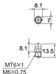
A-M6F (M6×0.75)
